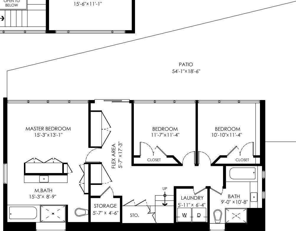
Lower Floor Plan Floor Area: 1189 sq.ft. Ceiling Height: 7'-6"
