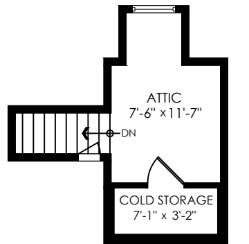
Upper Floor Plan Floor Area: 126 sq.ft. Ceiling Height: 5'-10" Vaulted
