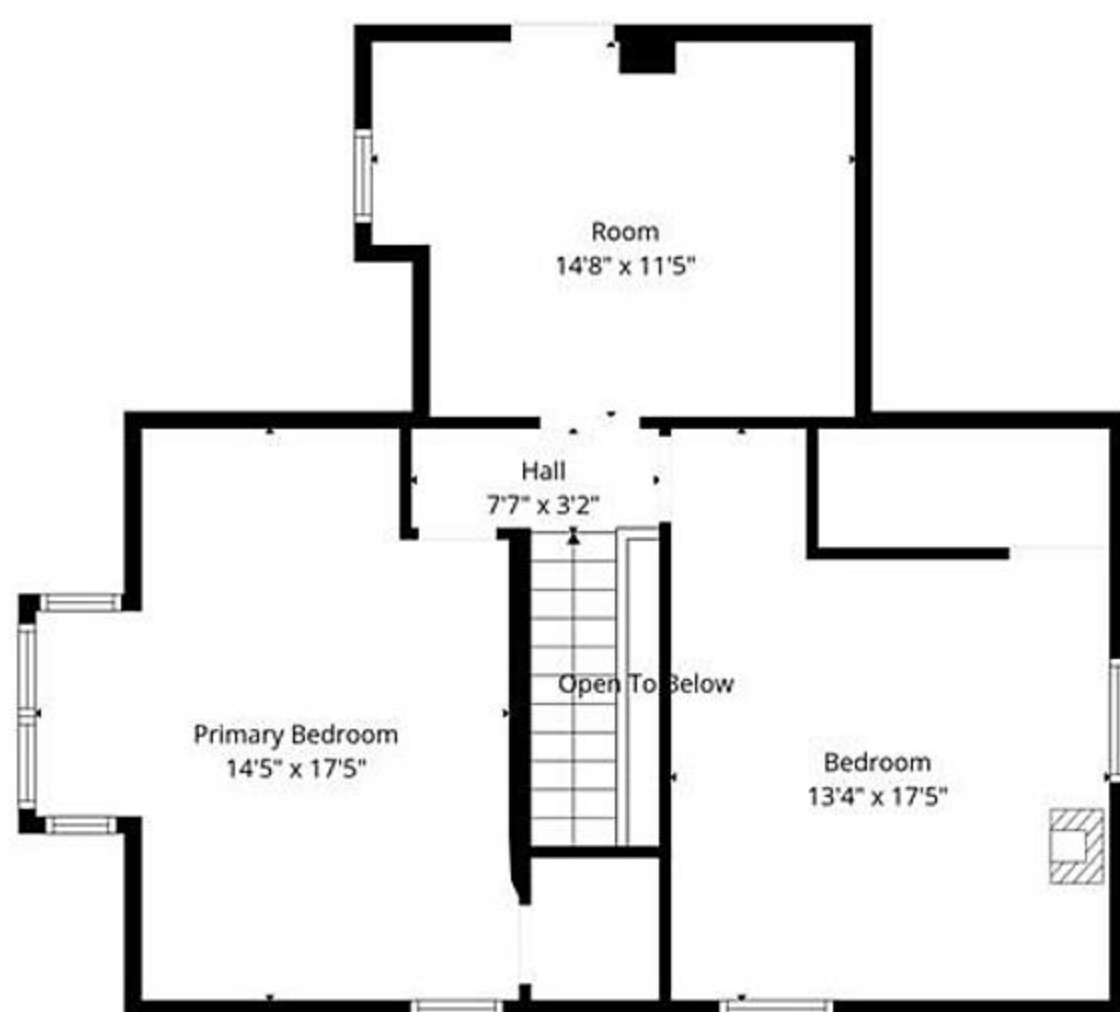
2nd Floor
