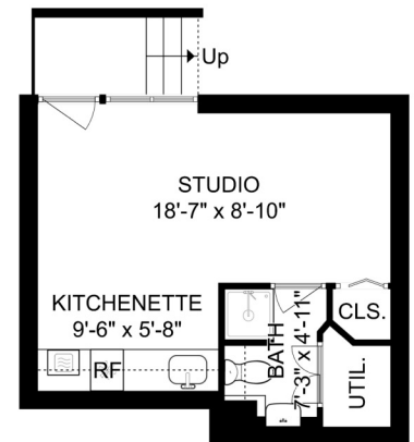
LOWER FLOOR 336 sq.ft. | Ceiling Height: 7'-0"
