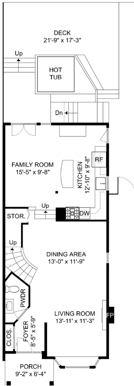
MAIN FLOOR 888 sq.ft. | Ceiling Height: 7'-9" to 9'-7"
