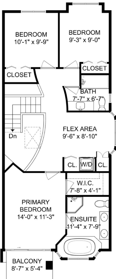
UPPER FLOOR 892 sq.ft. | Ceiling Height: 9'-0"
