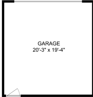
GARAGE 392 sq.ft. | Ceiling Height: 8'-10"
