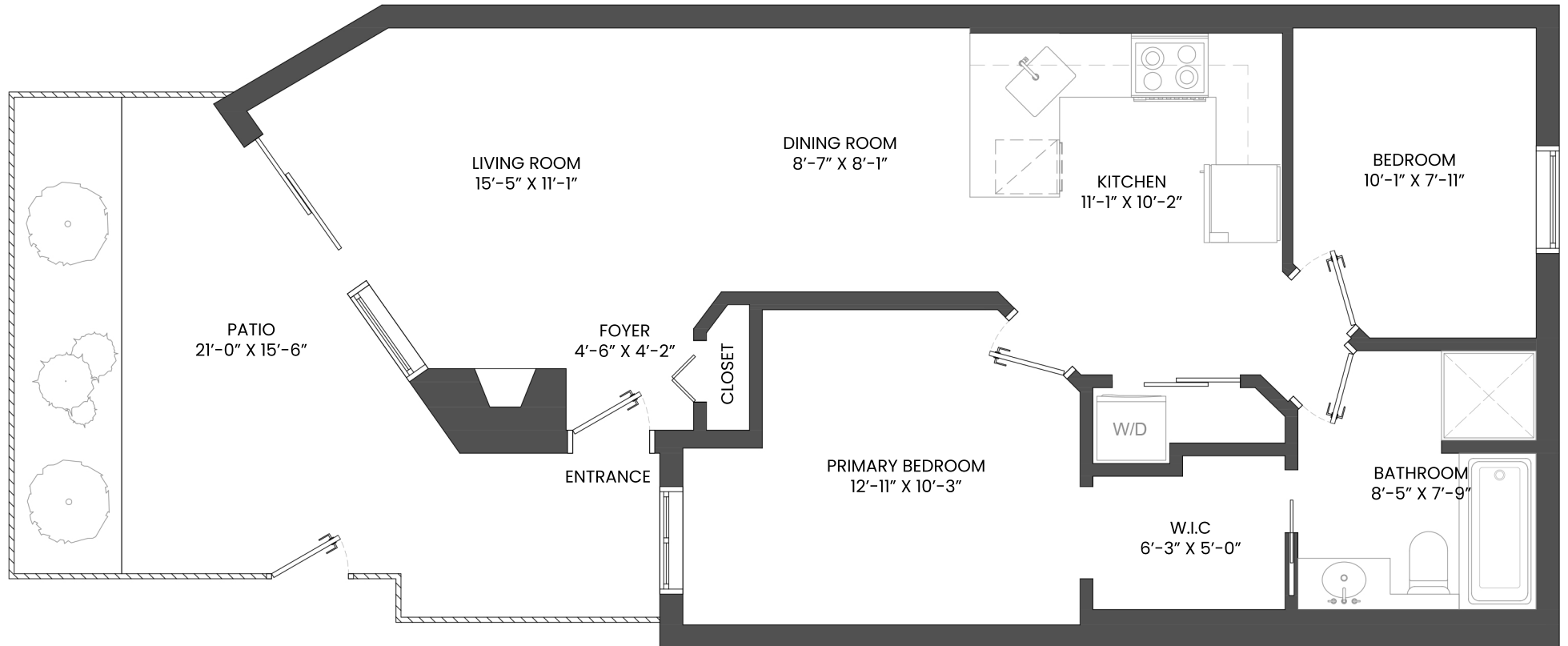
MAIN FLOOR PLAN Ceiling Height: 8'-0"
