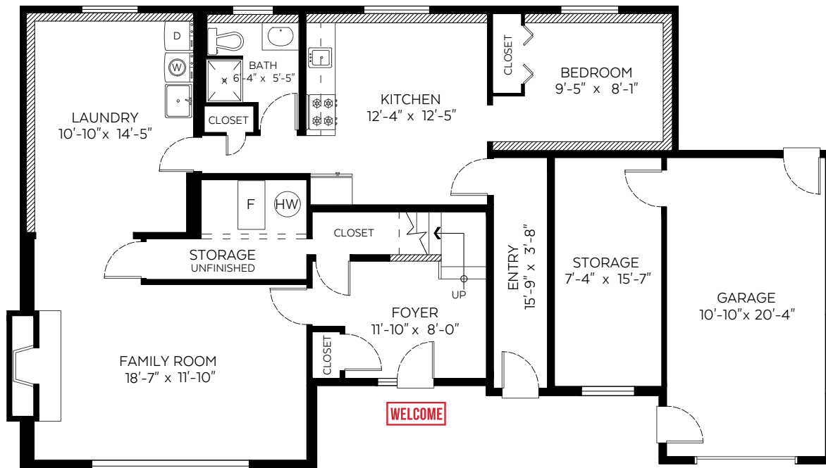
Lower Floor Plan
