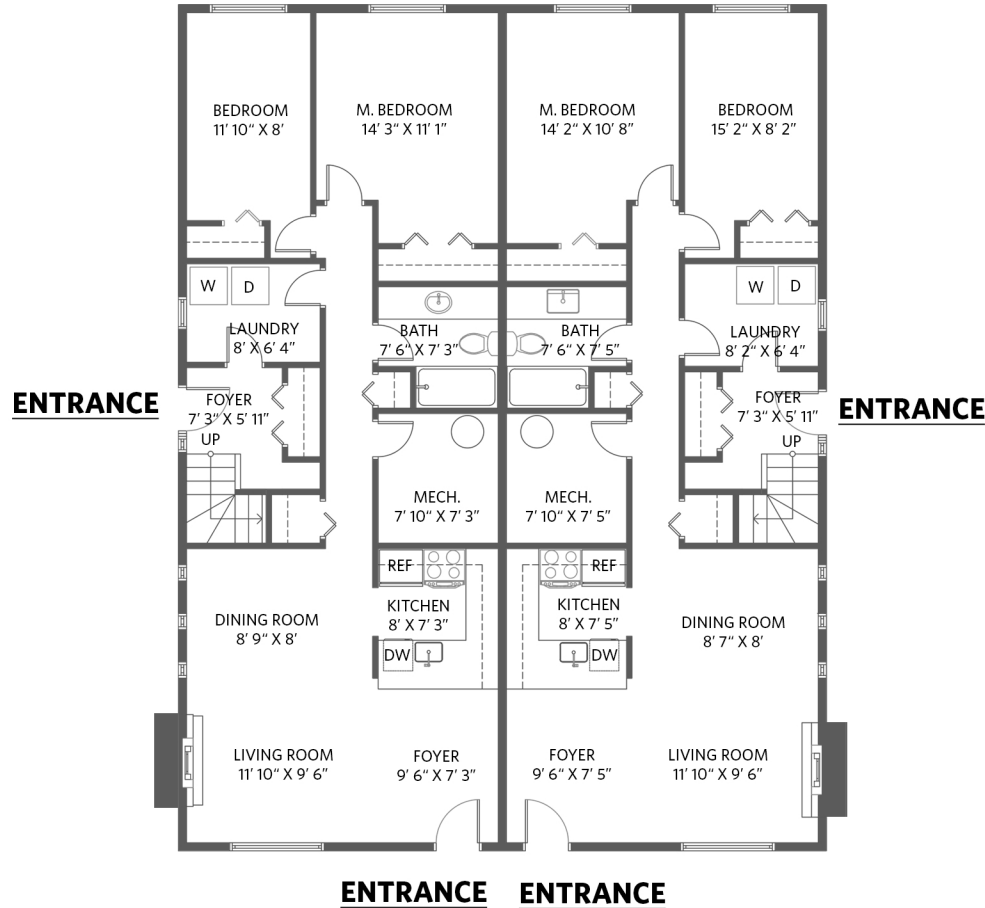
Main Floor - 2,110 sq.ft.
