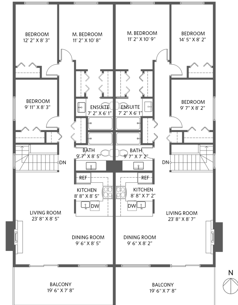
Upper Floor - 2,110 sq.ft.
