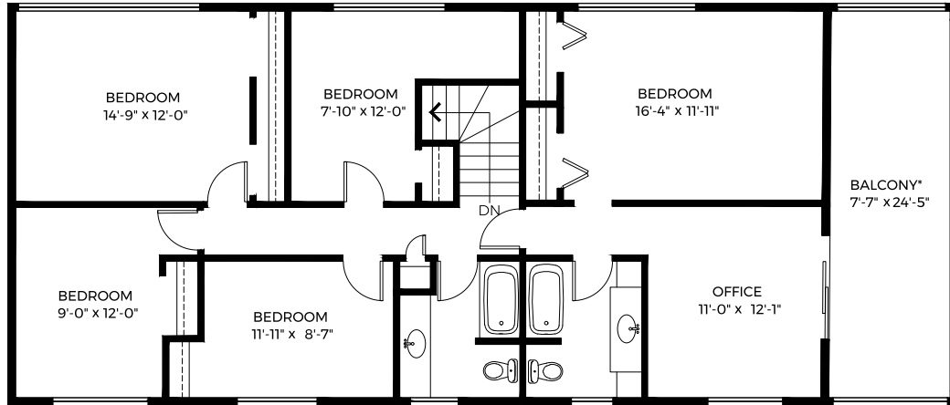
ABOVE MAIN
