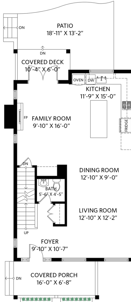
Main Floor - 870 sq.ft. Ceiling height - 9' 0"
