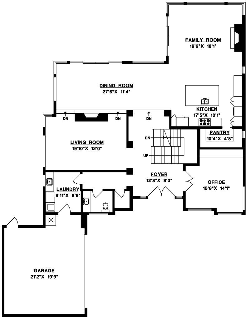
MAIN FLOOR
