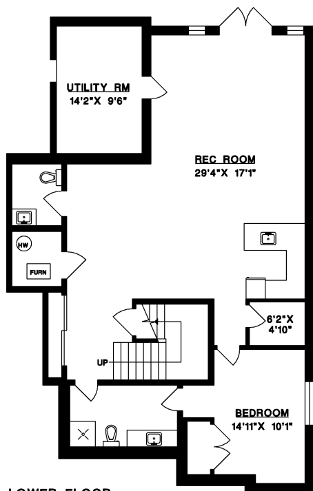
LOWER FLOOR
