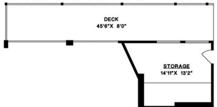
BOTTOM FLOOR
