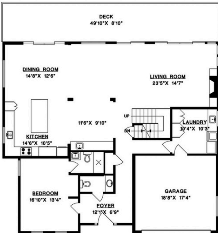
MAIN FLOOR
