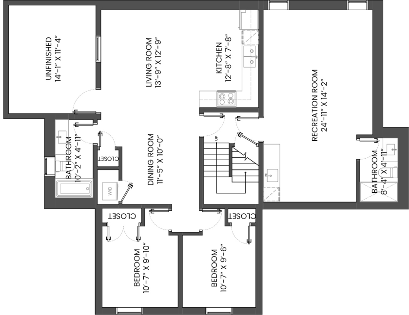
LOWER FLOOR PLAN Ceiling Height: 8'-0"
