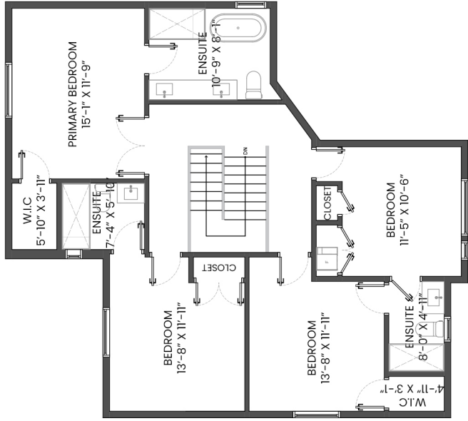
UPPER FLOOR PLAN Ceiling Height: 8'-0"
