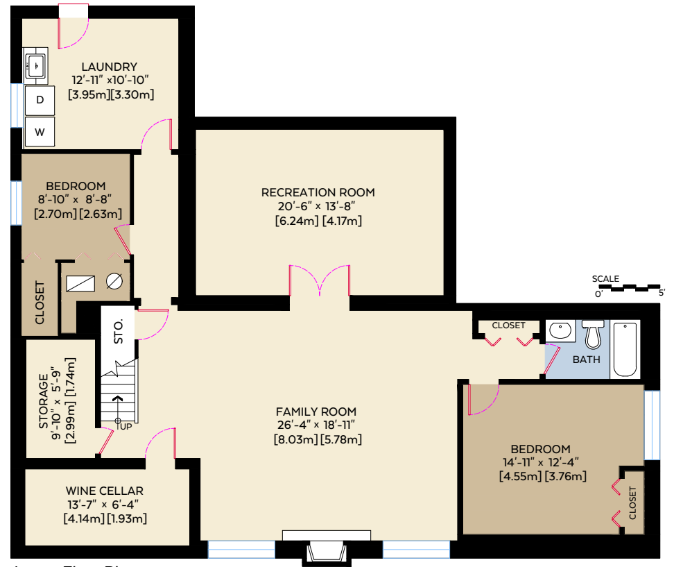
Lower Floor Plan Floor Area: 1,820 sq.ft. Floor Area: 169.08 sq.m.
