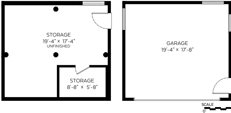
Sub-Main Floor Plan Floor Area: 664 sq.ft.
