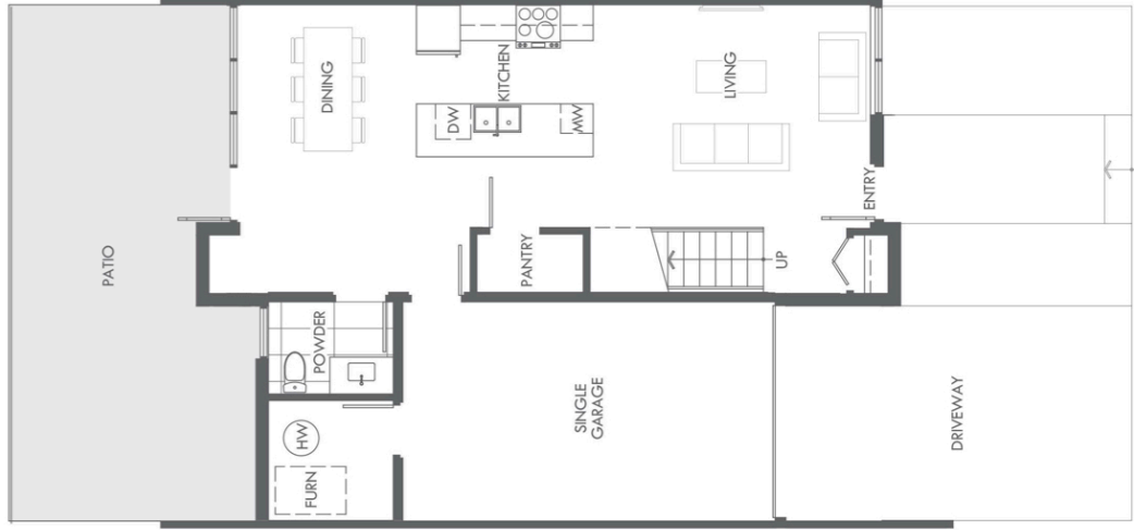
MAIN FLOOR
