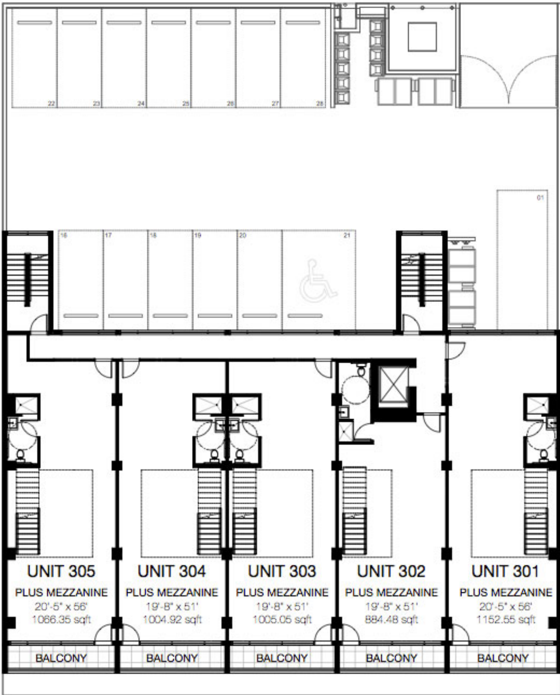
Third Floor 0 5 10 15 20 25 FT
