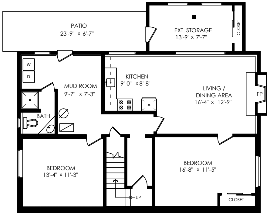
Lower Floor: 1071 Sq.Ft. Ceiling Height: 7'-11"
