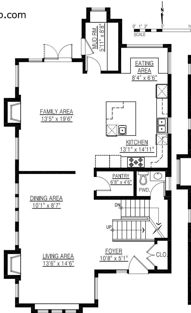
MAIN FLOOR PLAN FLOOR AREA: 1,216 sq.ft.
