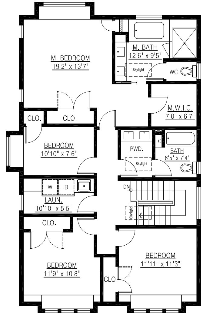
UPPER FLOOR PLAN FLOOR AREA: 1,208 sq.ft.
