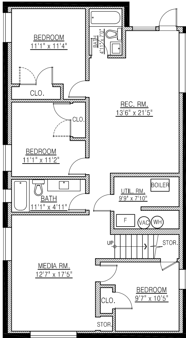
BASEMENT FLOOR PLAN FLOOR AREA: 1,362 sq.ft.
