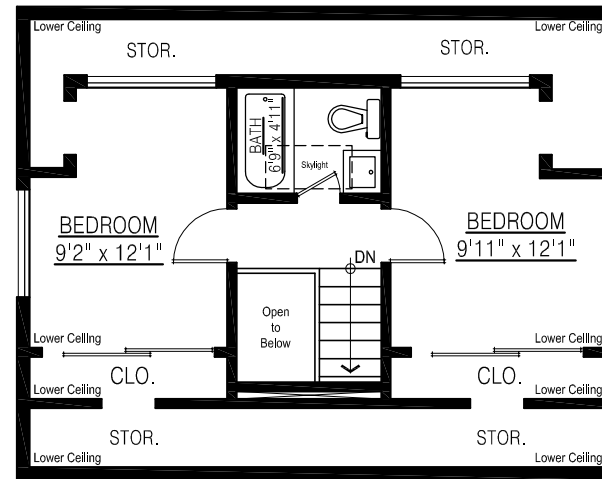
COACH HOUSE: UPPER FLOOR PLAN FLOOR AREA: *590 sq.ft.
