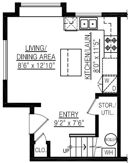
COACH HOUSE: MAIN FLOOR PLAN FLOOR AREA: 353 sq.ft.
