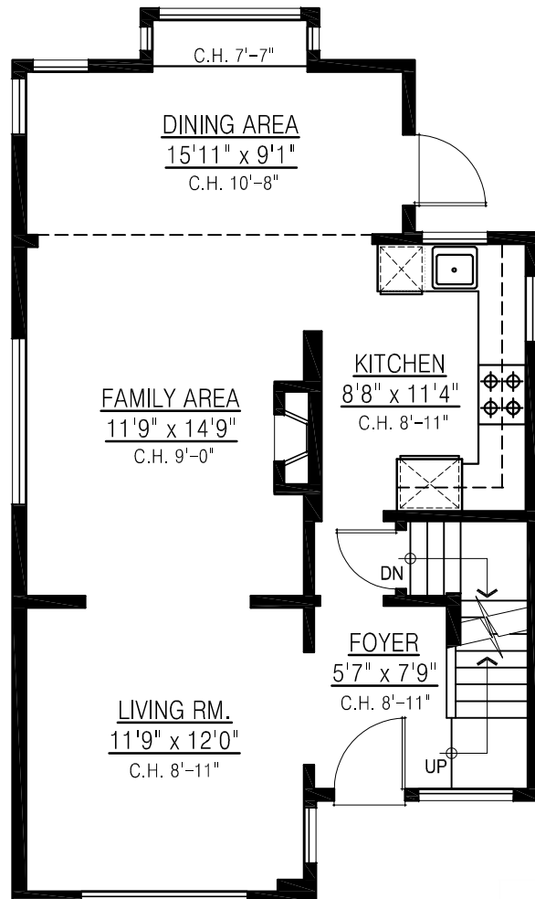
MAIN FLOOR PLAN FLOOR AREA: 732 sq.ft.
