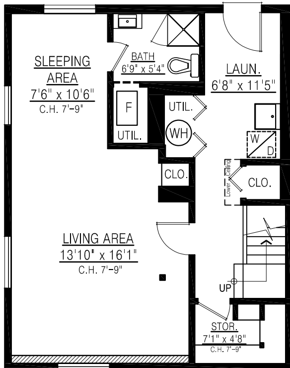
LOWER FLOOR PLAN FLOOR AREA: 633 sq.ft.
