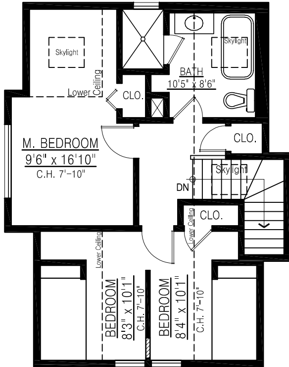
UPPER FLOOR PLAN FLOOR AREA: *551 sq.ft.
