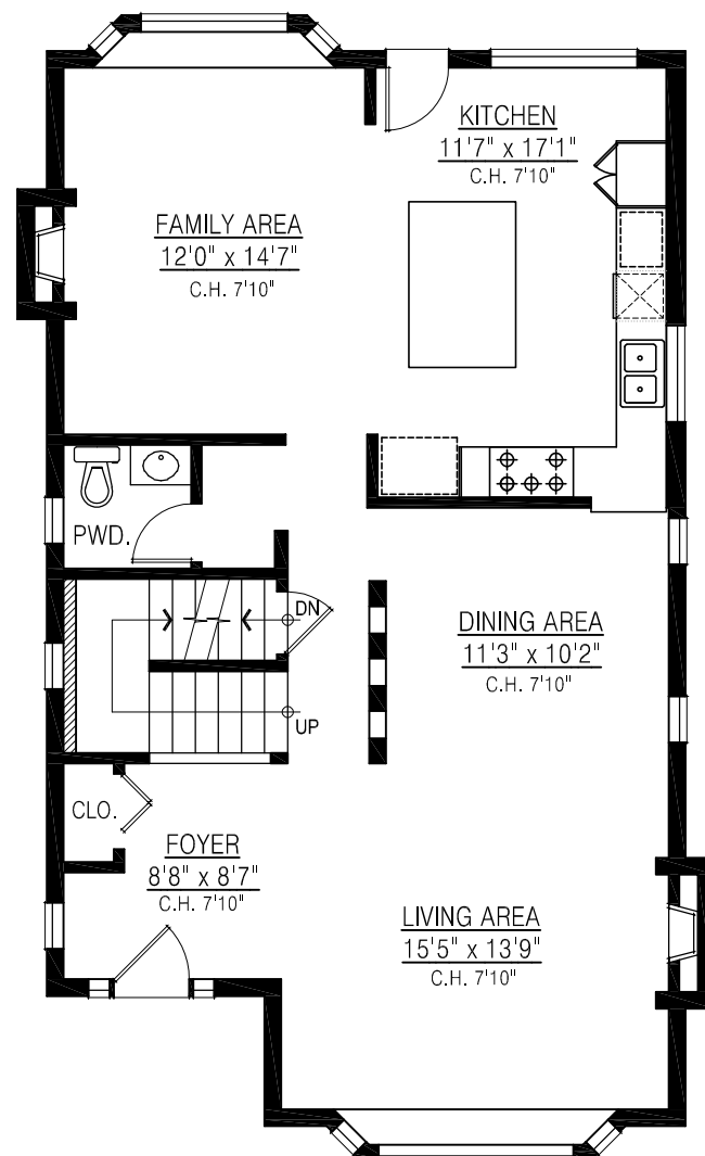
MAIN FLOOR PLAN FLOOR AREA: 1,042 sq.ft.
