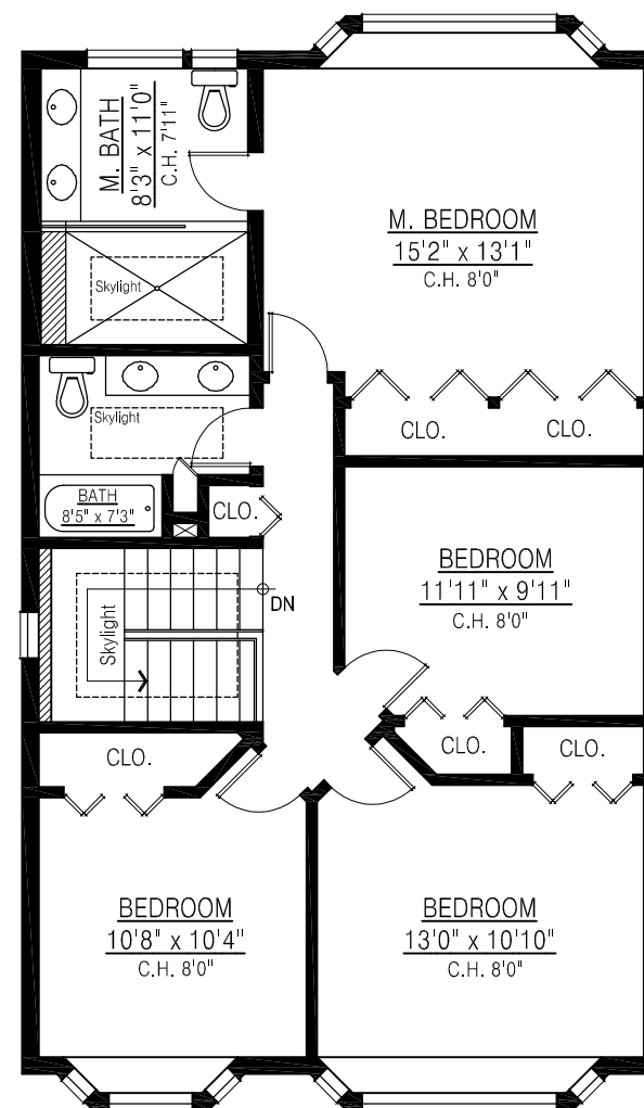
UPPER FLOOR PLAN FLOOR AREA: 972 sq.ft.
