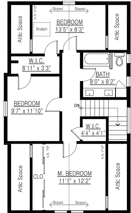
UPPER FLOOR PLAN FLOOR AREA: *833 sq.ft. C.H. 7'8"
