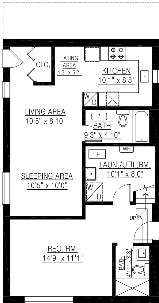
LOWER FLOOR PLAN FLOOR AREA: 851 sq.ft. C.H. 7'8"
