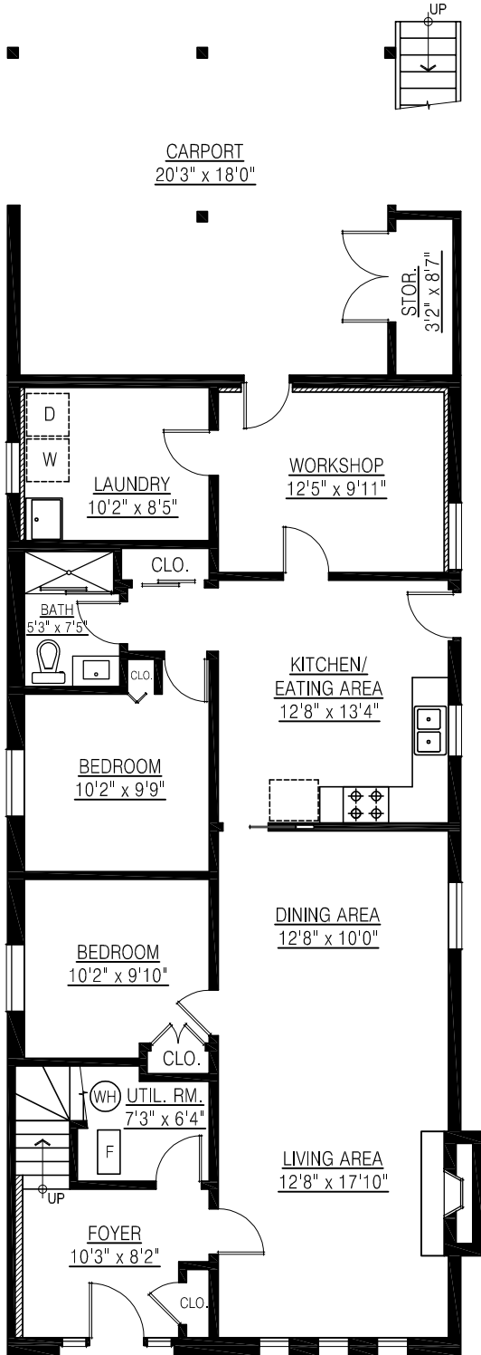
LOWER FLOOR PLAN FLOOR AREA: 1,318 sq.ft. C.H.:7'-11"
