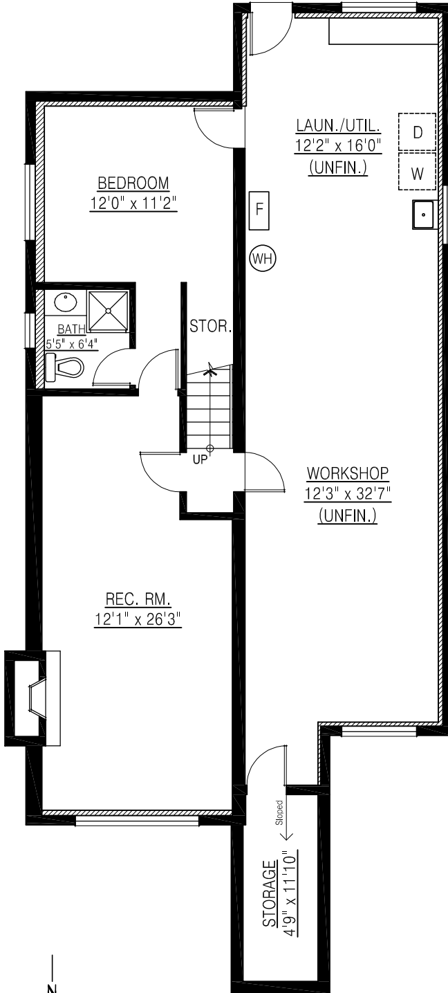
BASEMENT FLOOR PLAN FLOOR AREA: **1,319 sq. ft. C.H.: 8'-0"
