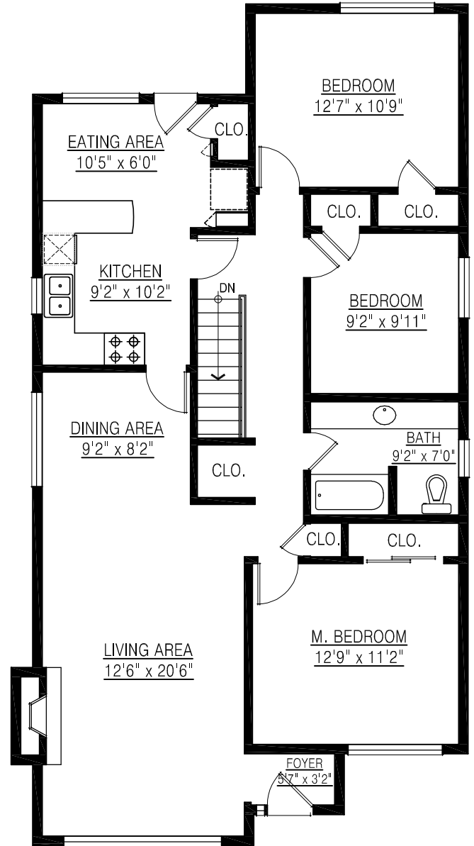
MAIN FLOOR PLAN FLOOR AREA: 1,272 sq. ft. C.H.: 7'-5"
