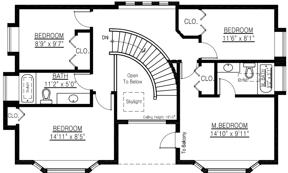
UPPER FLOOR PLAN FLOOR AREA: 891 sq.ft. CEILING HEIGHT: 8'-0"
