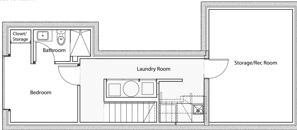
Basement Floorplan
