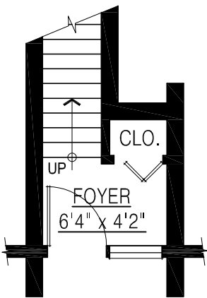
ENTRY FLOOR PLAN FLOOR AREA: 67 sq.ft. CH:7'-11"
