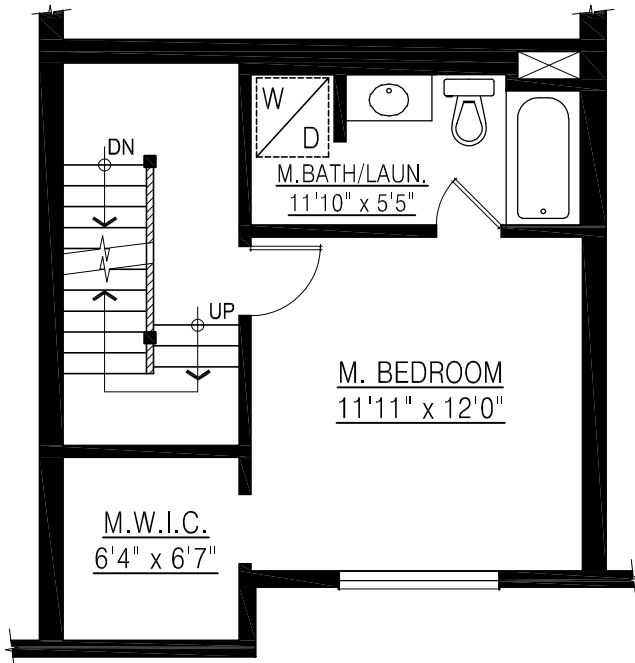
LOWER FLOOR PLAN FLOOR AREA: 371 sq.ft. CH:7'-11"
