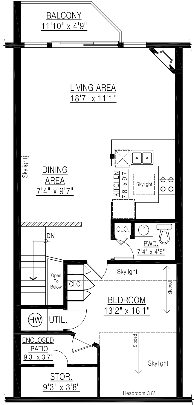
MAIN FLOOR PLAN FLOOR AREA: *760 sq.ft. CH:7'-11"
