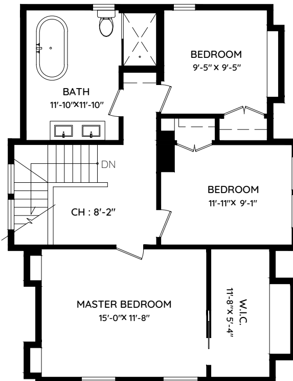
UPPER FLOOR 841 SQ.FT. CH: 8'-2"
