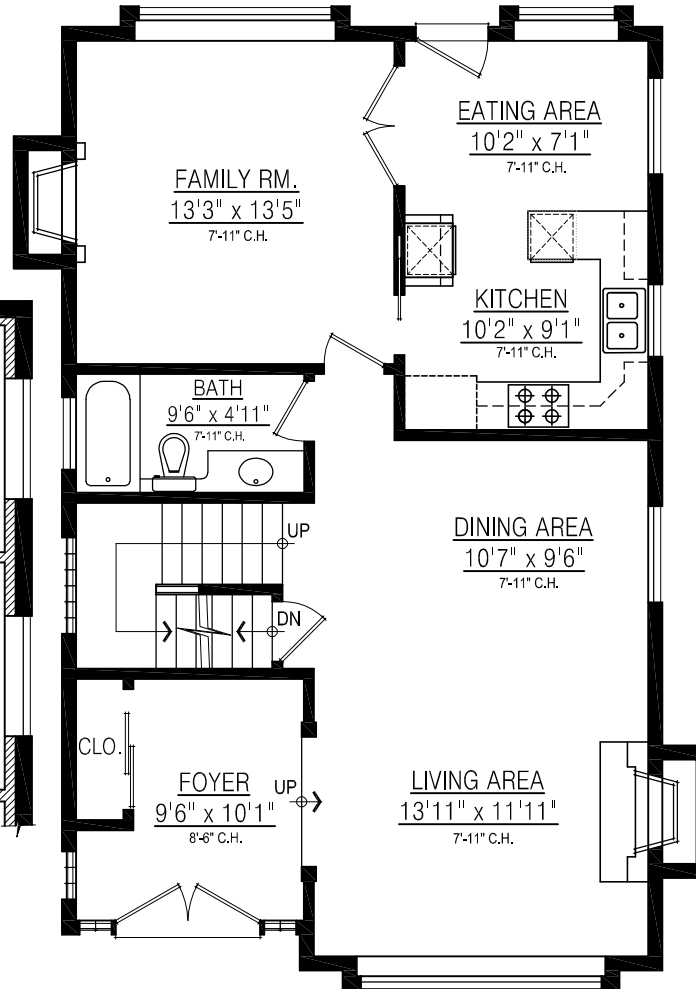
MAIN FLOOR PLAN FLOOR AREA: 963 sq.ft.
