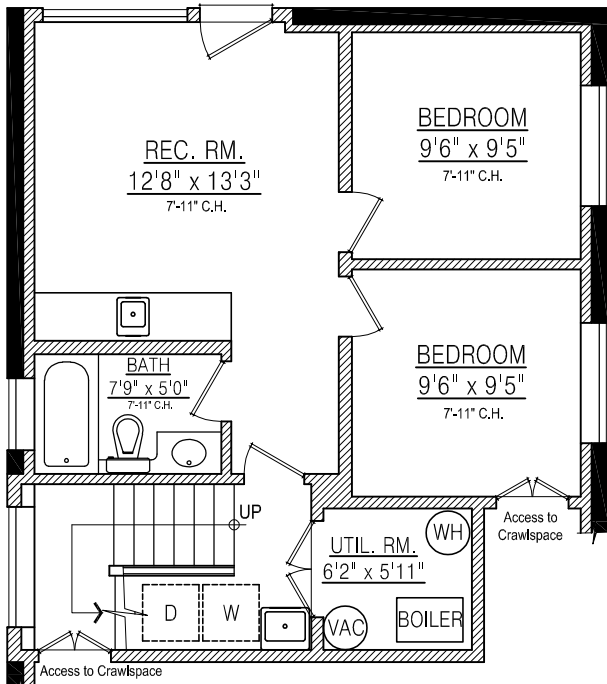
BASEMENT FLOOR PLAN FLOOR AREA: 645 sq.ft.
