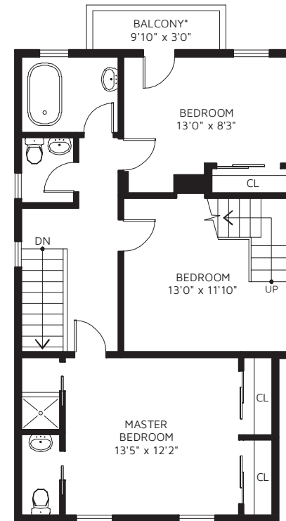
UPPER FLOOR
