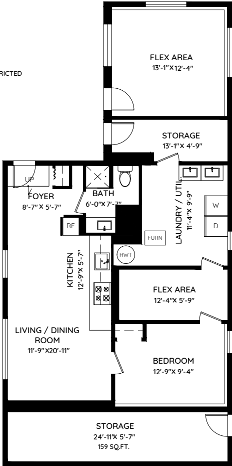
LOWER FLOOR 1,003 SQ.FT. CH: 8'-0"
