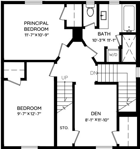
UPPER FLOOR 751 SQ.FT. CH: 8'-3"
