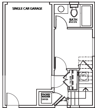
LANEWAY HOUSE LOWER FLOOR PLAN
