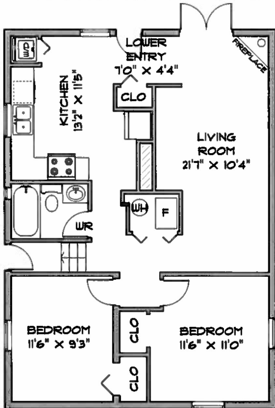
LOWER LEVEL 866 SQ. FT.
