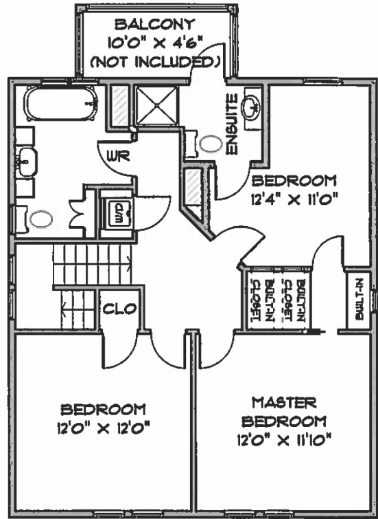
UPPER LEVEL 750 SQ. FT.
