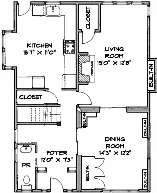
MAIN LEVEL 909 SQ. FT.
