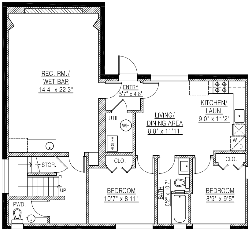
BASEMENT FLOOR PLAN FLOOR AREA: 1,182 sq.ft.
