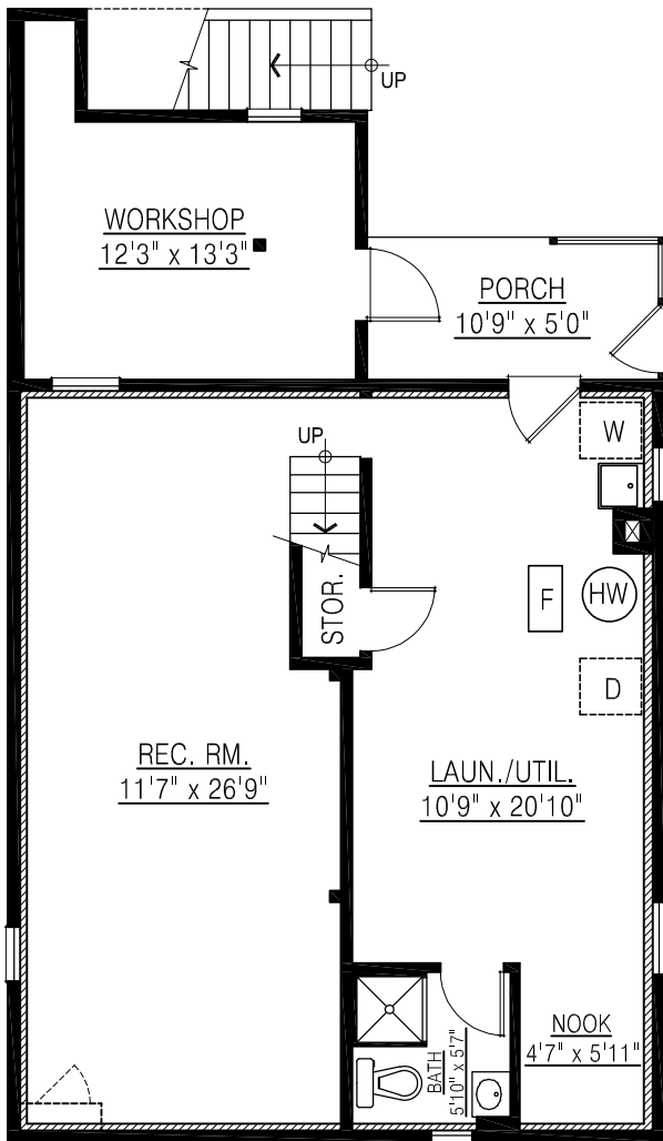
BASEMENT PLAN FLOOR AREA: 667 sq. ft. C.H. = 6'-2"
