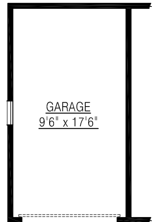
GARAGE FLOOR PLAN FLOOR AREA: 186 sq. ft.
