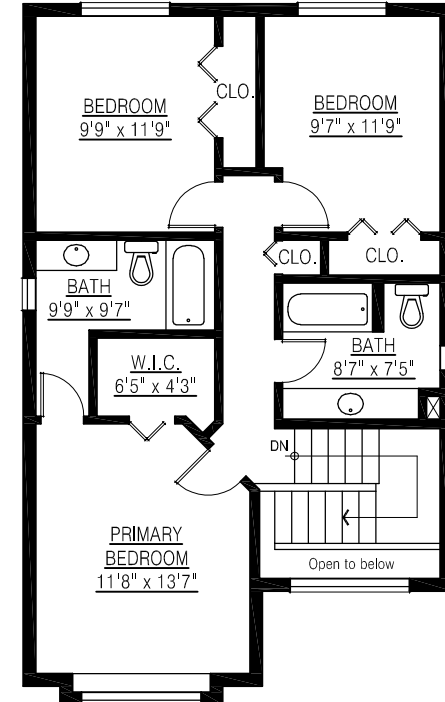
UPPER FLOOR PLAN FLOOR AREA: 738 sq.ft. C.H.: 8'-0"
