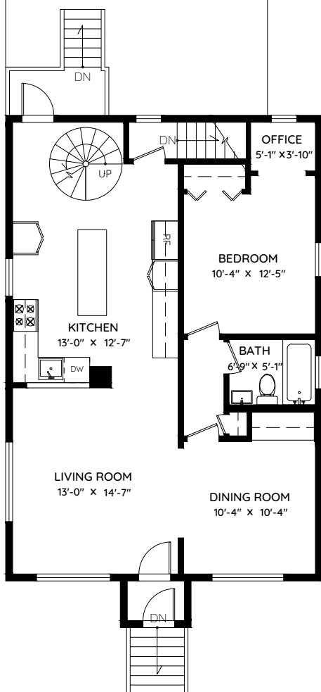
MAIN FLOOR 925 SQ.FT. CH: 8'-2"
