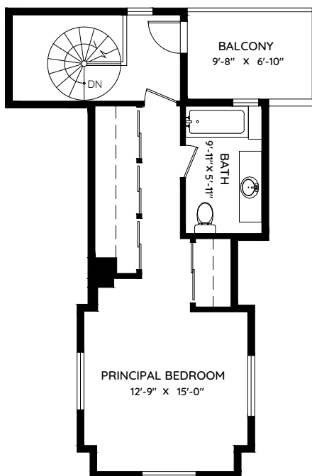
UPPER FLOOR 406 SQ.FT. CH: 6'-9"
