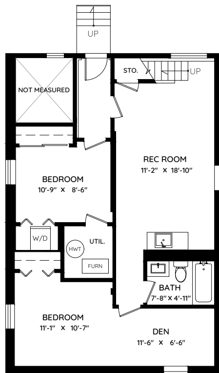
LOWER FLOOR 845 SQ.FT. CH: 7'-0"
