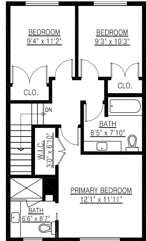
UPPER FLOOR PLAN FLOOR AREA: 652 sq.ft. C.H.: 8'-0"
