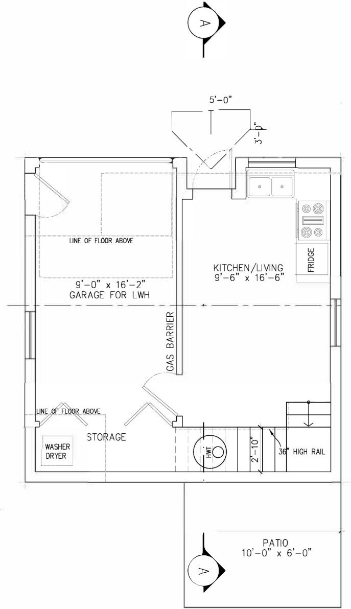
FIRST STORY AND FOUNDATION PLAN (371.35 SQ.FT.) SCALE: 1/4" = 1'-0"
