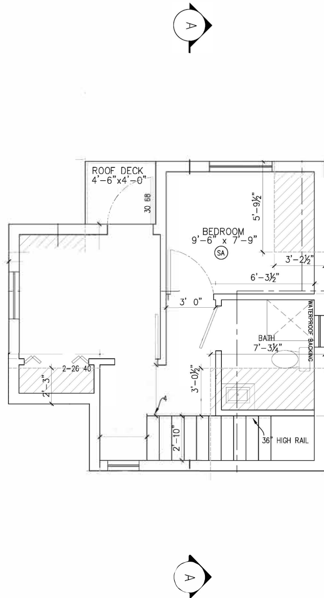
SECOND STORY (245.83 SQ.FT.) SCALE: 1/4" = 1'-0"
