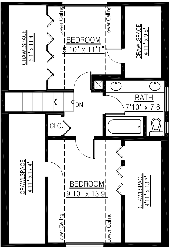
UPPER FLOOR PLAN FLOOR AREA: *405 sq.ft.
