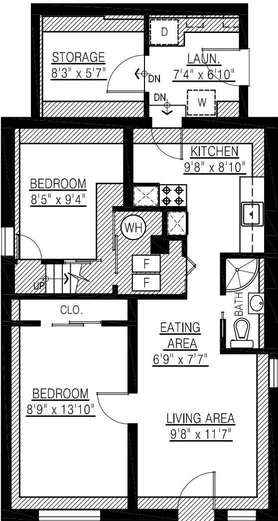
LOWER FLOOR PLAN FLOOR AREA: 726 sq.ft.
