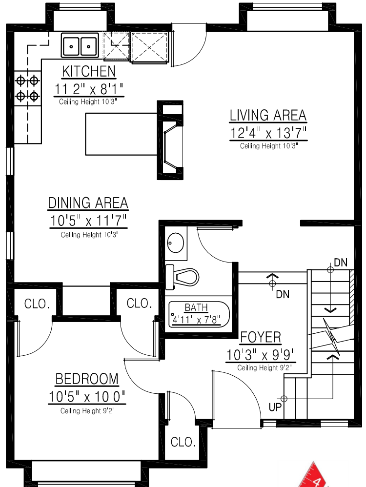
MAIN FLOOR PLAN FLOOR AREA: 778 sq.ft.
