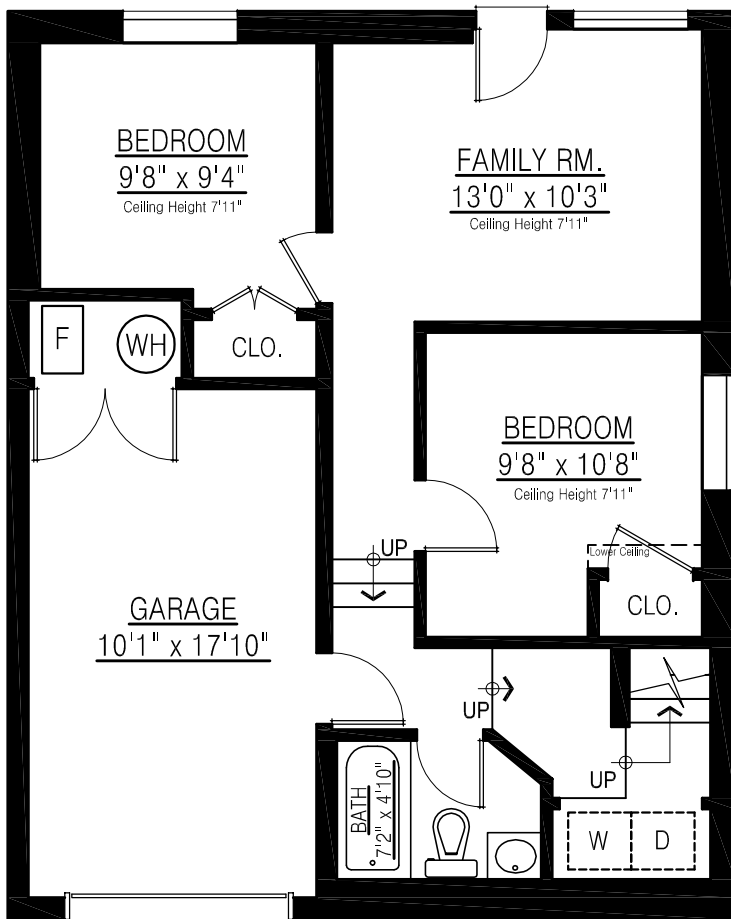
LOWER FLOOR PLAN FLOOR AREA: 590 sq.ft.
