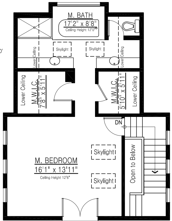
UPPER FLOOR PLAN FLOOR AREA: *567 sq.ft.
