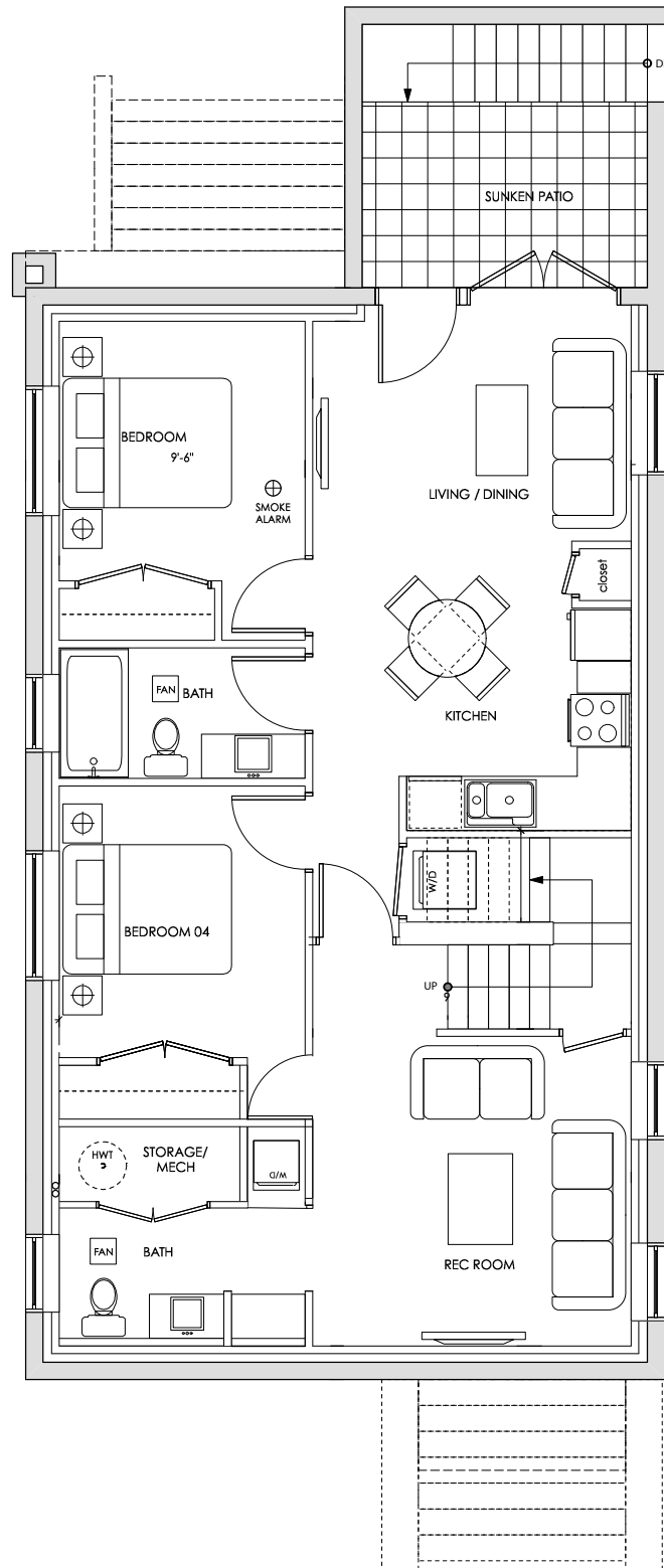
LOWER LEVEL FLOOR PLAN
