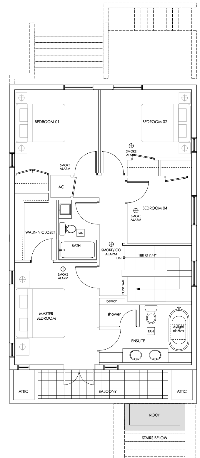
UPPER LEVEL FLOOR PLAN
