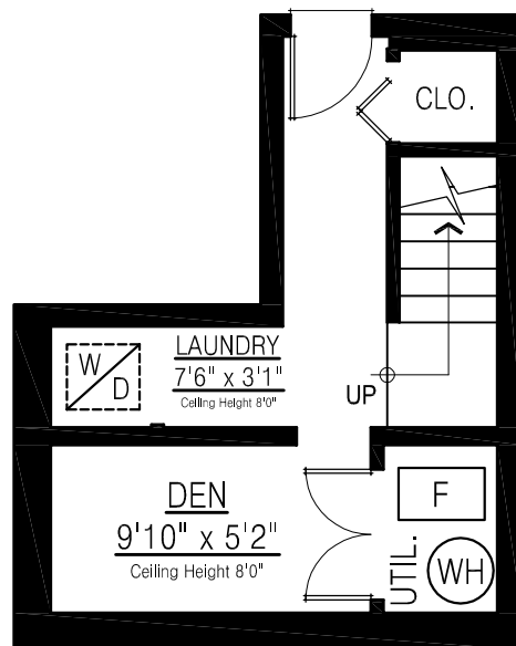
LOWER FLOOR PLAN FLOOR AREA: 228 sq.ft.
