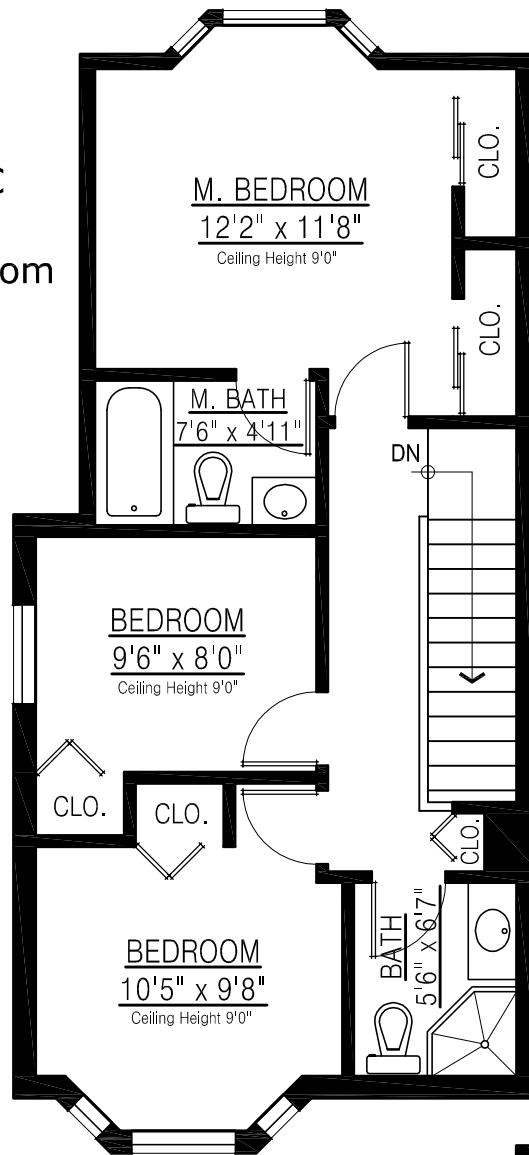
UPPER FLOOR PLAN FLOOR AREA: 593 sq.ft.
