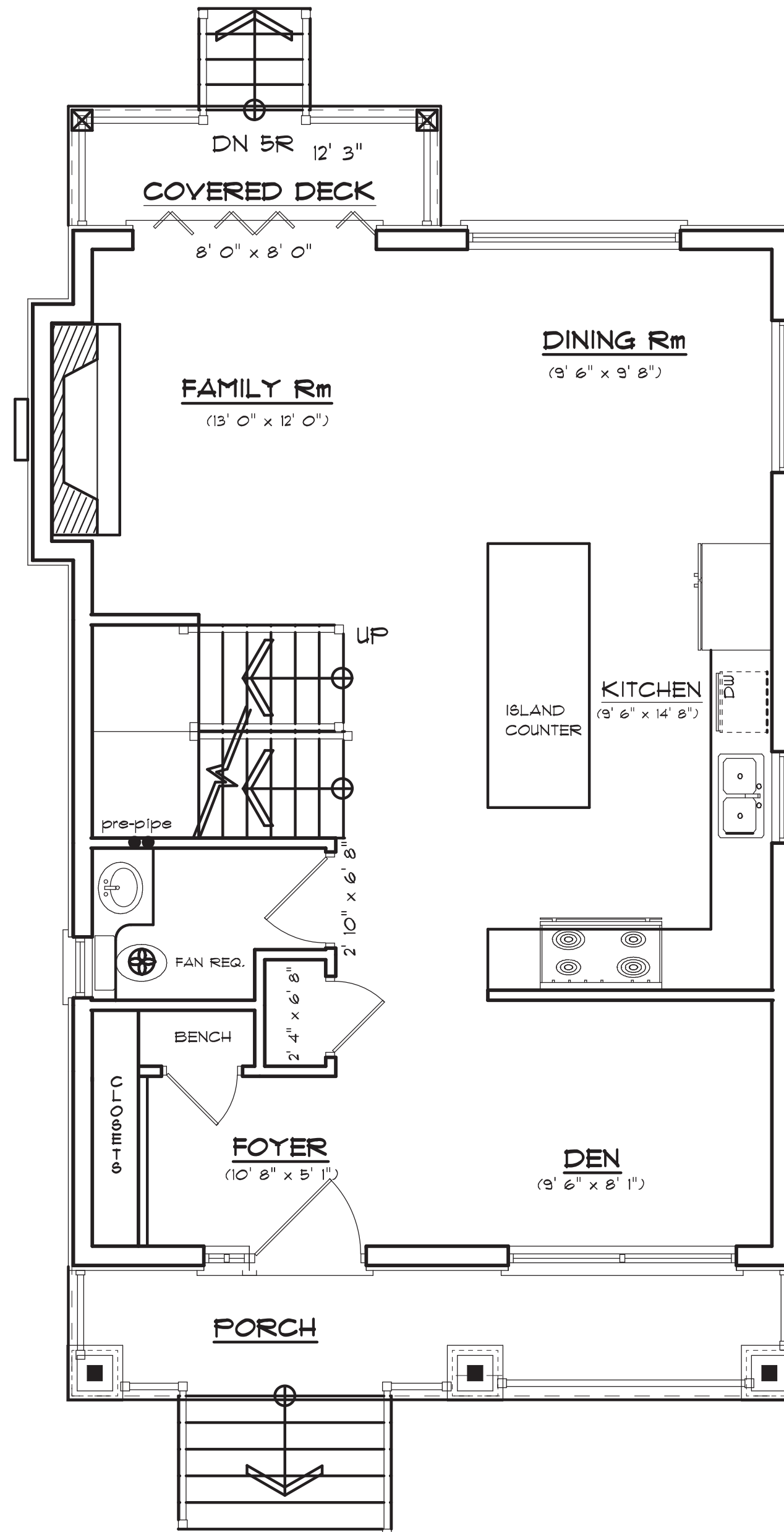
MAIN FLOOR - 842 SQFT
