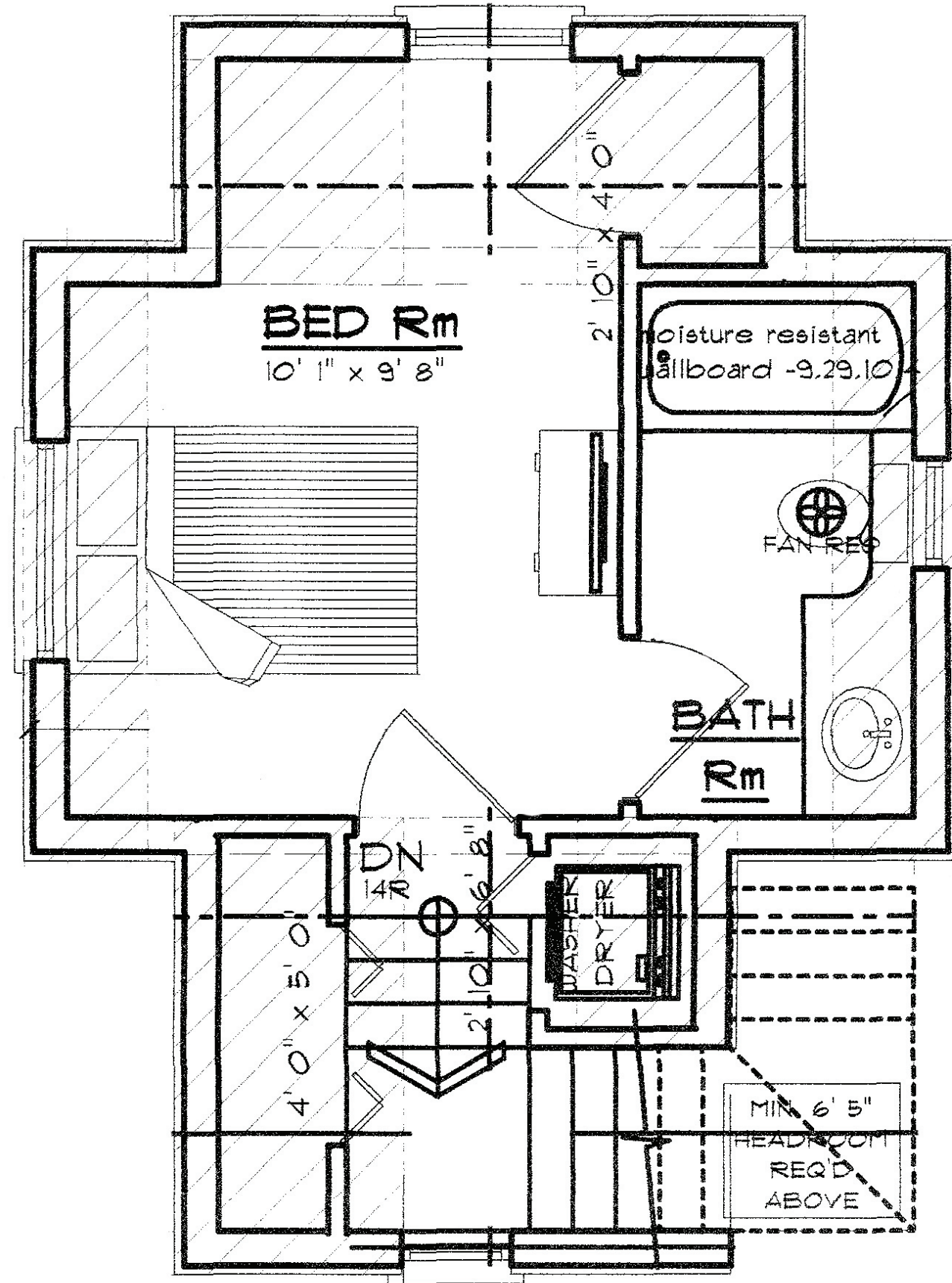
SECOND FLOOR - 227 SQFT
