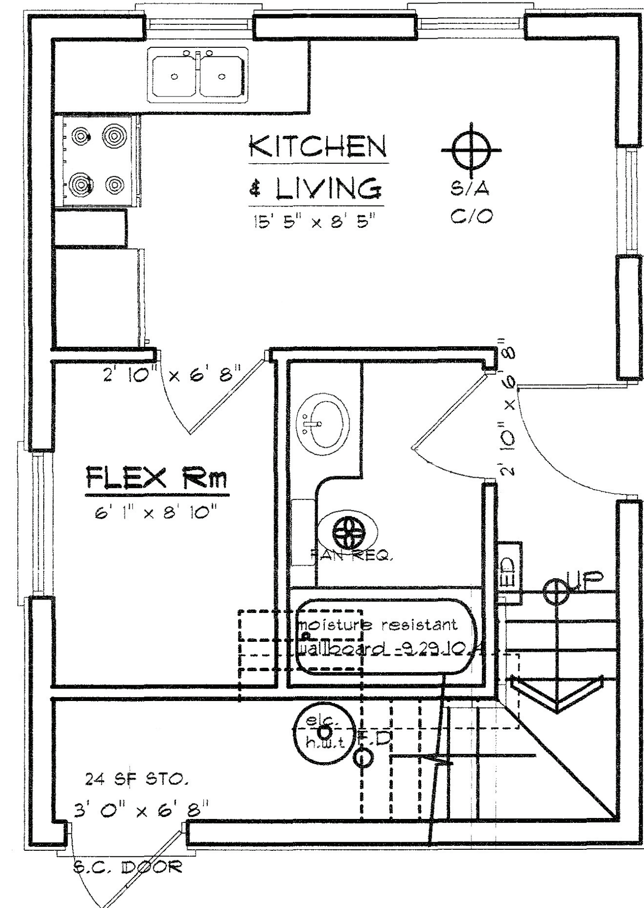
MAIN FLOOR - 364 SQFT
