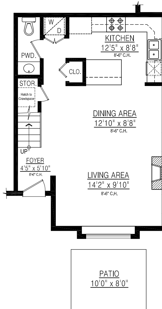
MAIN FLOOR PLAN FLOOR AREA: 551 sq.ft.
