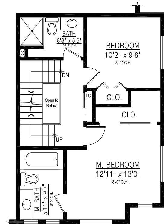
UPPER FLOOR PLAN FLOOR AREA: 549 sq.ft.
