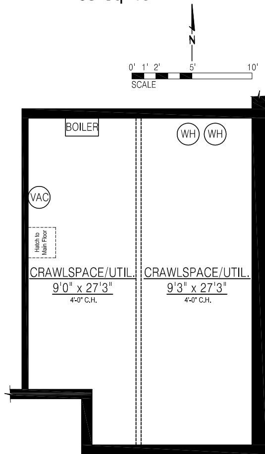
CRAWLSPACE PLAN FLOOR AREA: 550 sq.ft.
