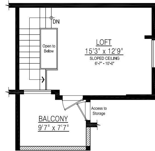
TOP FLOOR PLAN FLOOR AREA: 239 sq.ft.
