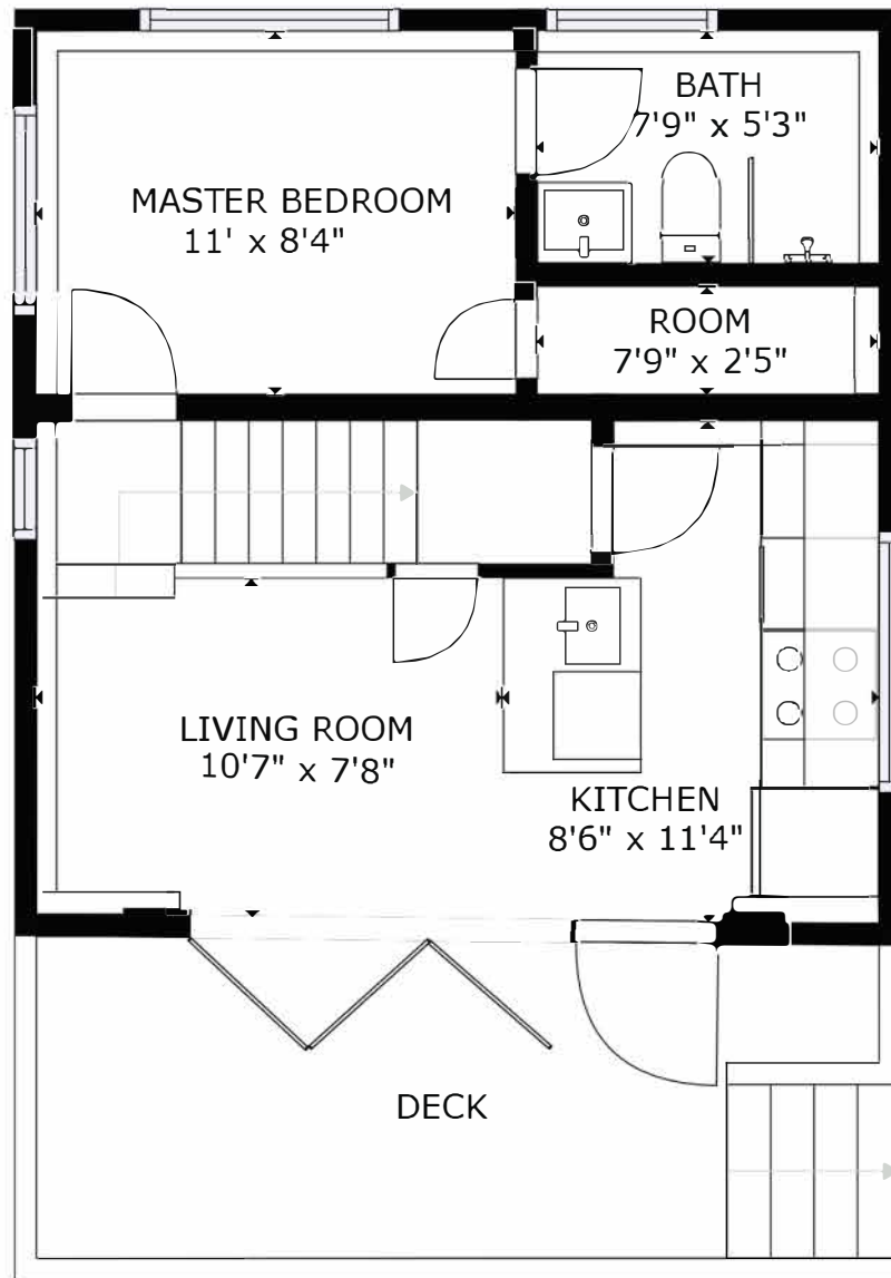
FLOOR 1
