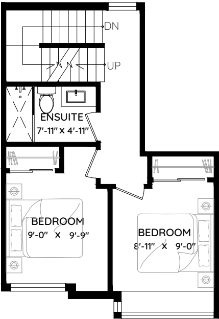
TOP FLOOR 485 SQ.FT. CH: 8'-0"
