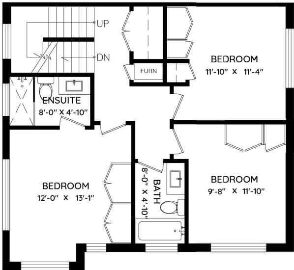
UPPER FLOOR 729 SQ.FT. CH: 8'-5"
