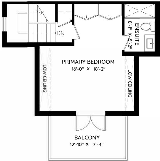
TOP FLOOR 419 SQ.FT. CH: 9'-7" (VAULTED)
