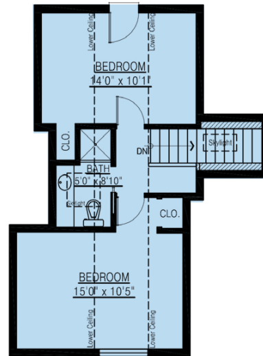
UPPER FLOOR PLAN FLOOR AREA: *513 sq.ft.
